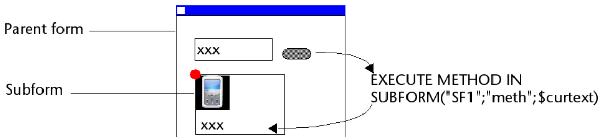
Example of execution of EXECUTE METHOD IN SUBFORM command
